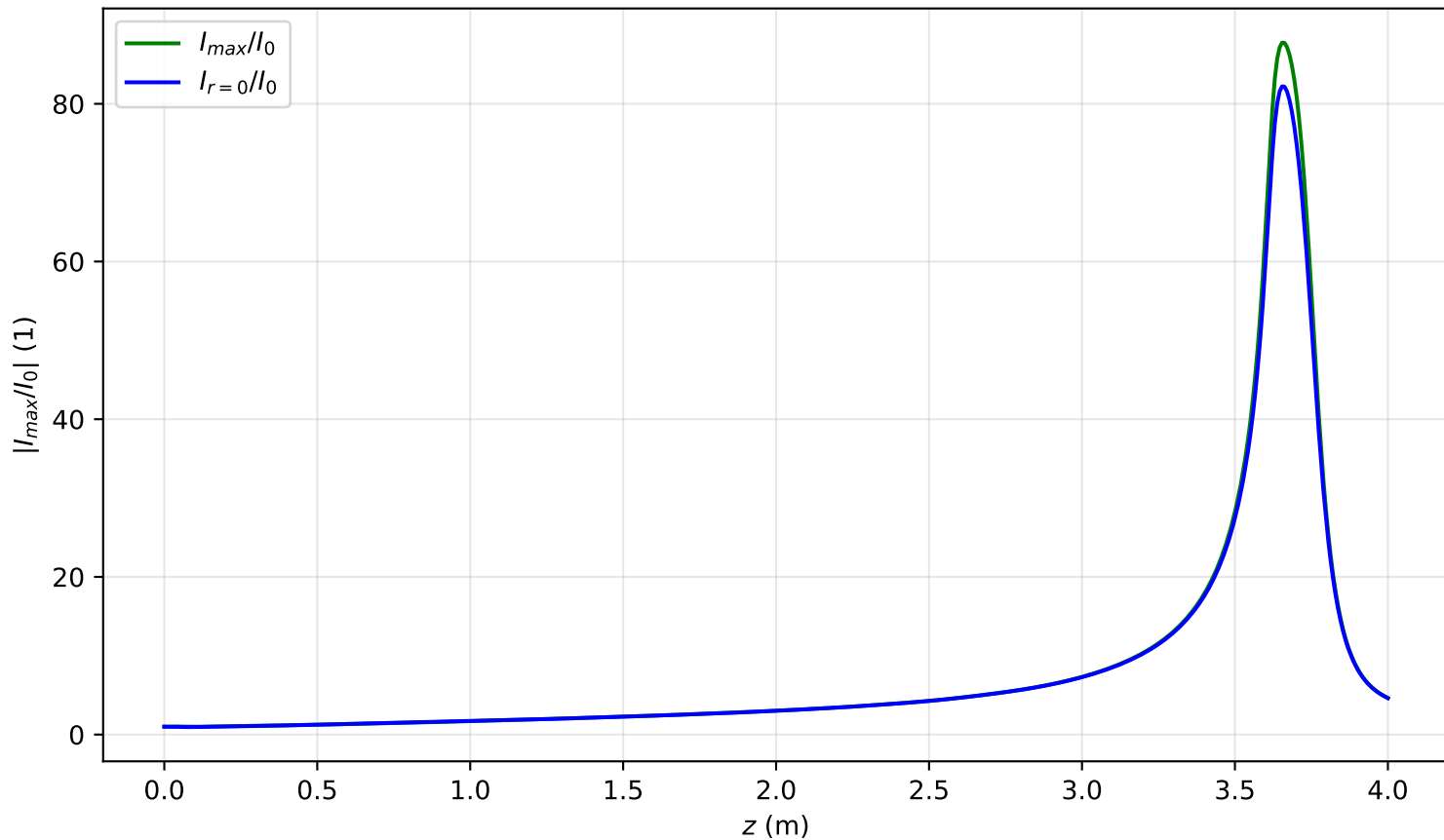
I_{max}(x = 0, y = 0, z)/I_0 , P_{in}=1.1P_{cr} , noisy input, artificial time
